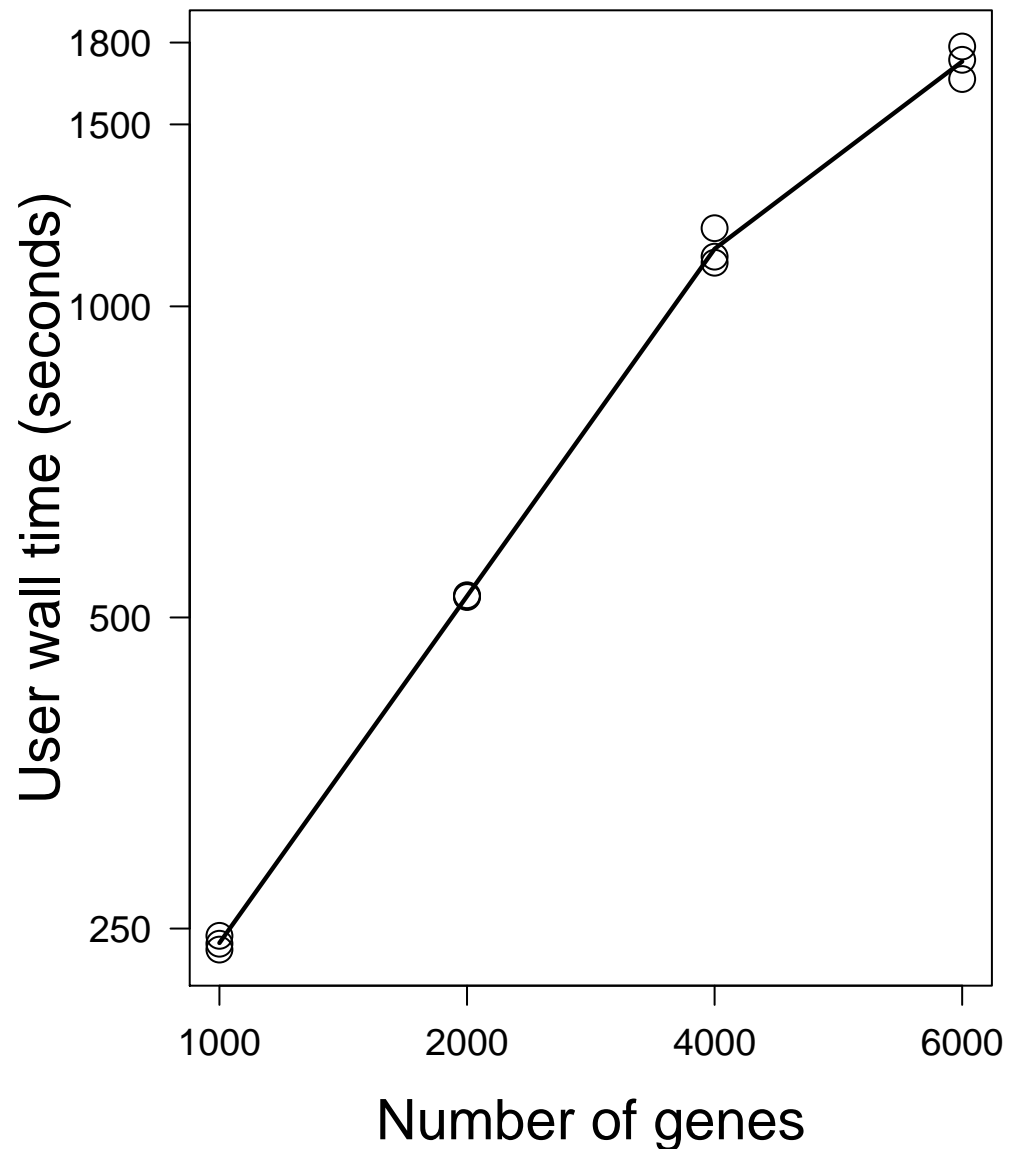
Prostate data set, 102 arrays
